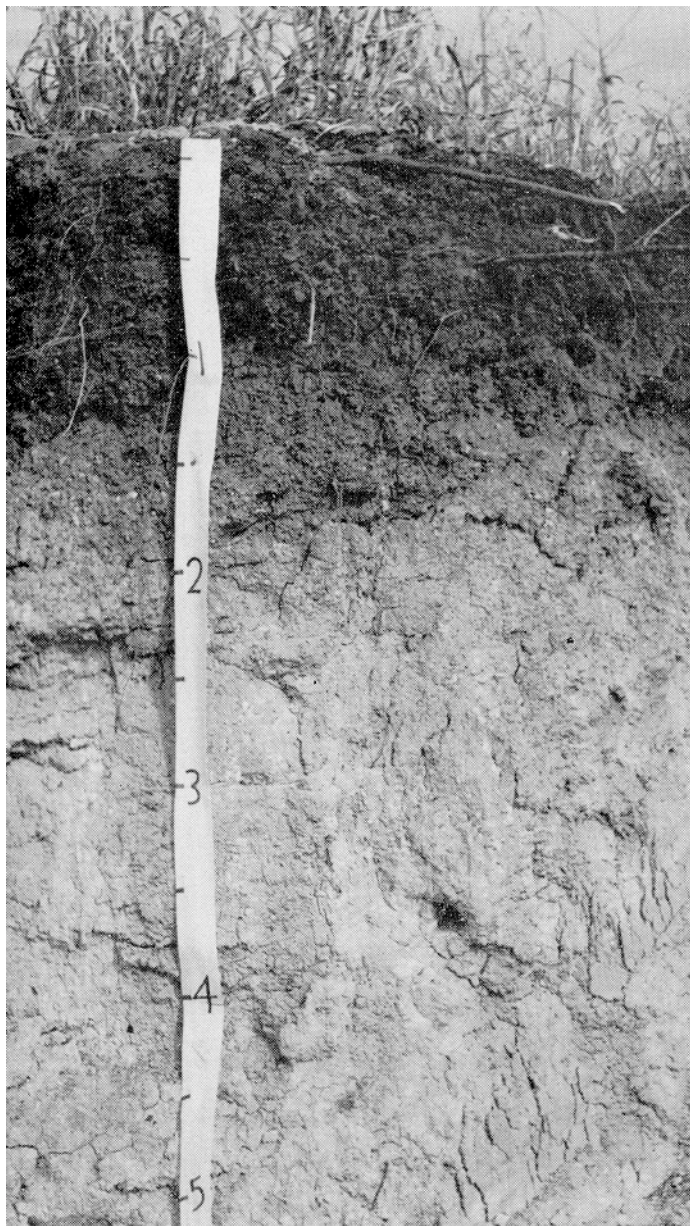
Figure 14.—Profile of Lewisville silty clay, showing a zone of lime accumulation at a depth of about 2 feet.
