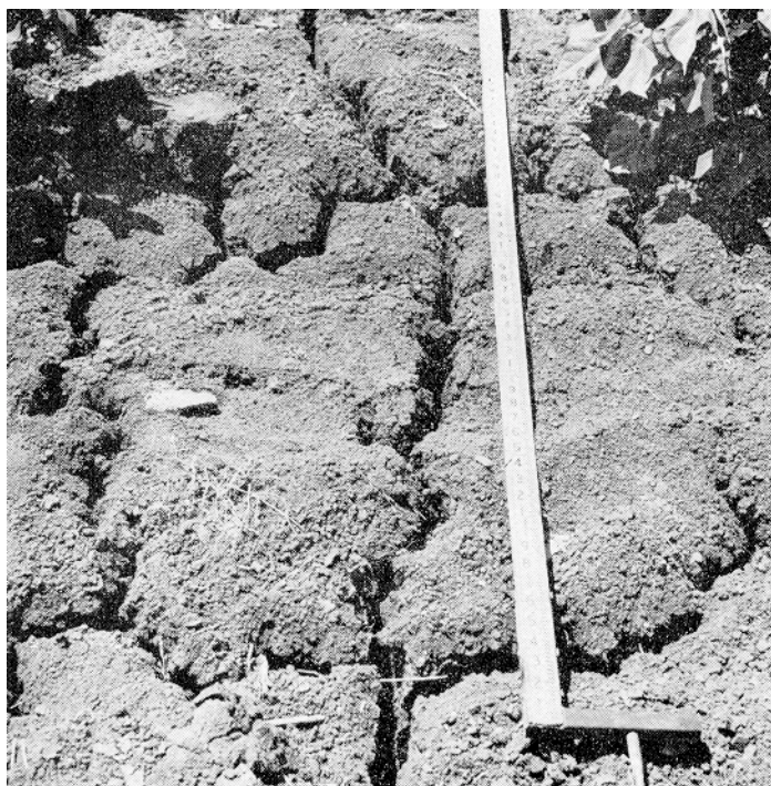
Figure 12.—Surface of Houston Black clay, 0 to 1 percent slopes, showing wide deep cracks and mulch of fine, discrete, very hard aggregates.
