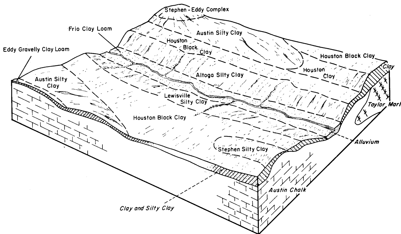
Figure 2.—Soils and underlying material in association 1.
