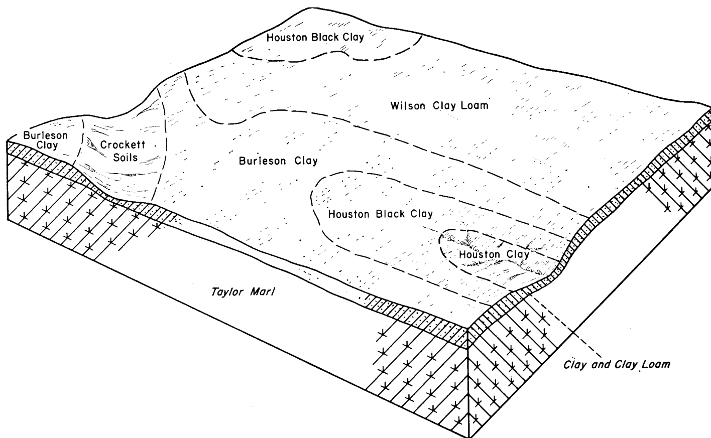
Figure 6.—Soils and underlying material in association 6.
