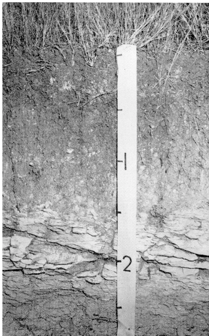
Figure 15.—Profile of a Stephen silty clay. A distinct layer of chalky limestone is at a depth of about 20 inches.
