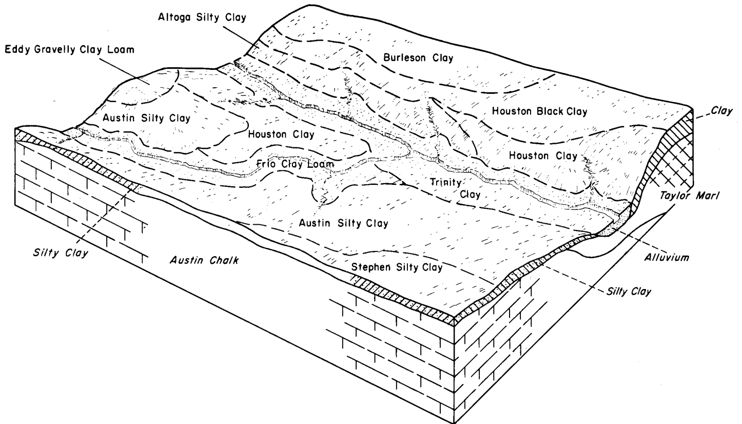
Figure 4.—Soils and underlying material in association 3.
