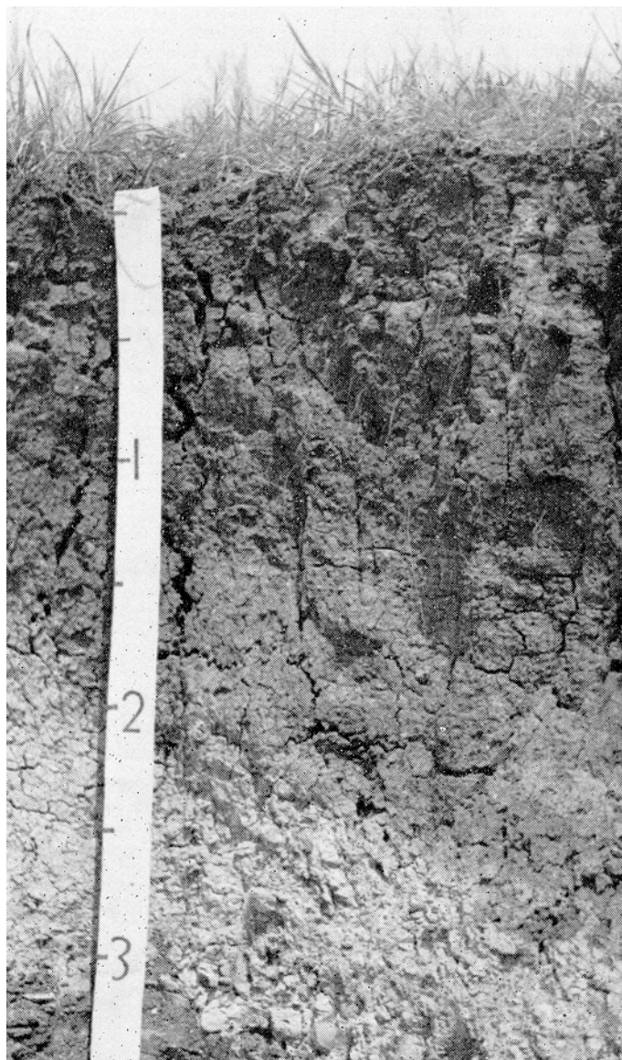
Figure 9.—Profile of Ferris clay. The C horizon of clayey marl is at a depth of 2 feet.
