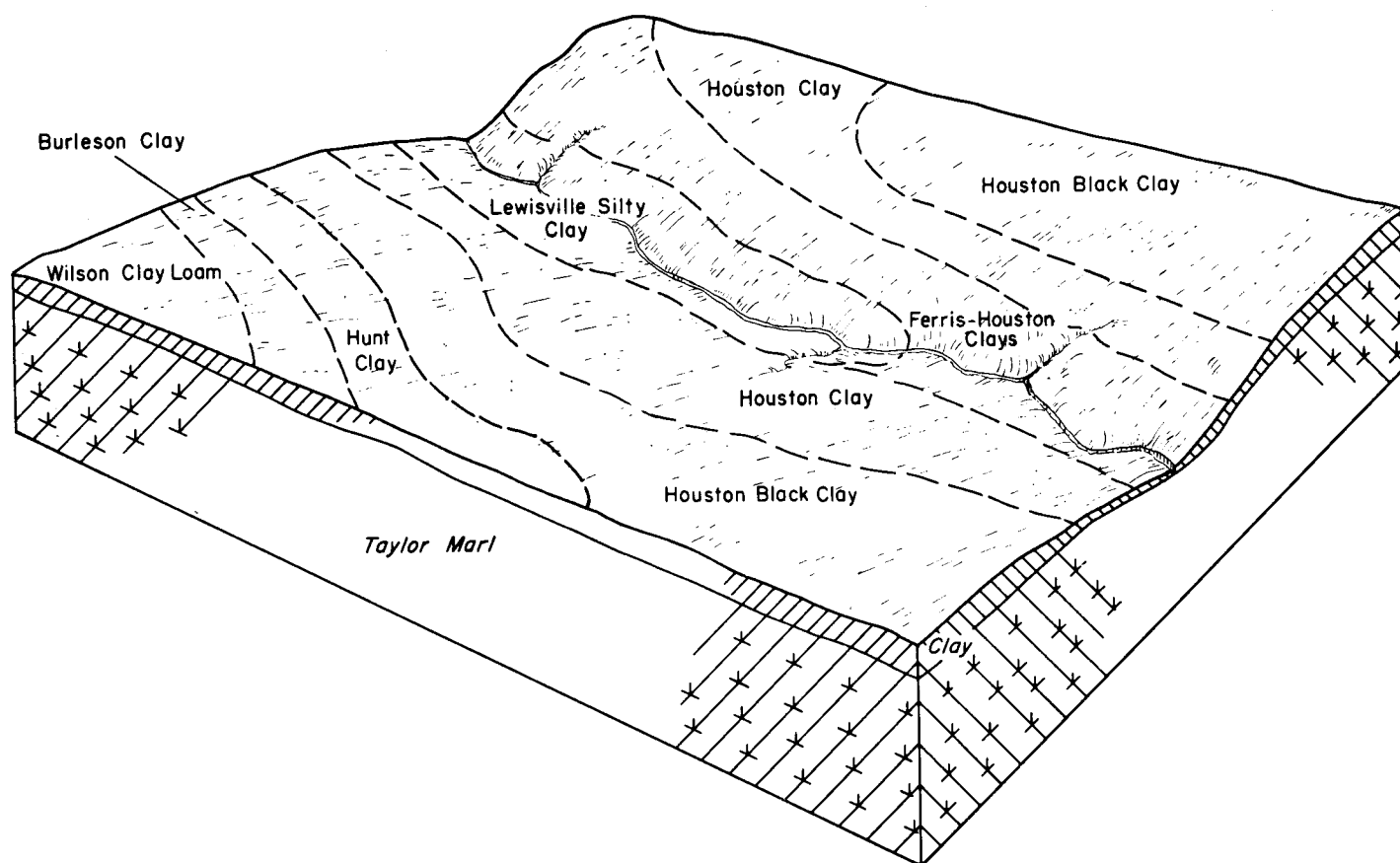
Figure 3.—Soils and underlying material in association 2.
