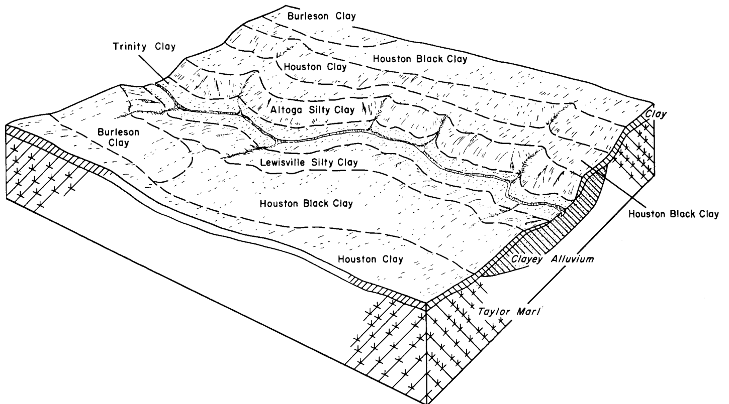
Figure 5.—Soils and underlying material in association 4.
